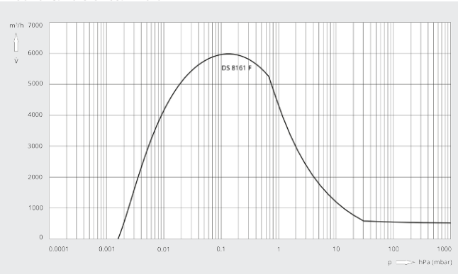
Pumping speed
