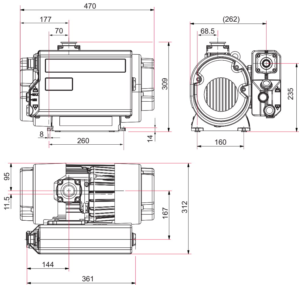
Fig. 19: Dimensions of SmartVane 70 Dimensions in mm
