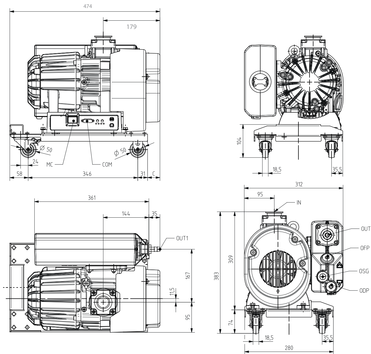
Fig. 20: Dimensions of SmartVane 55 with trolley Dimensions in mm
