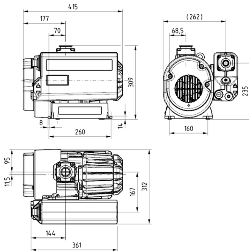
Fig. 18: Dimensions of SmartVane 55 with 1 l separator Dimensions in mm
