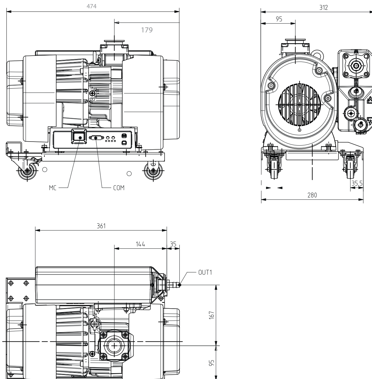
Fig. 21: Dimensions of SmartVane 70 with trolley Dimensions in mm
