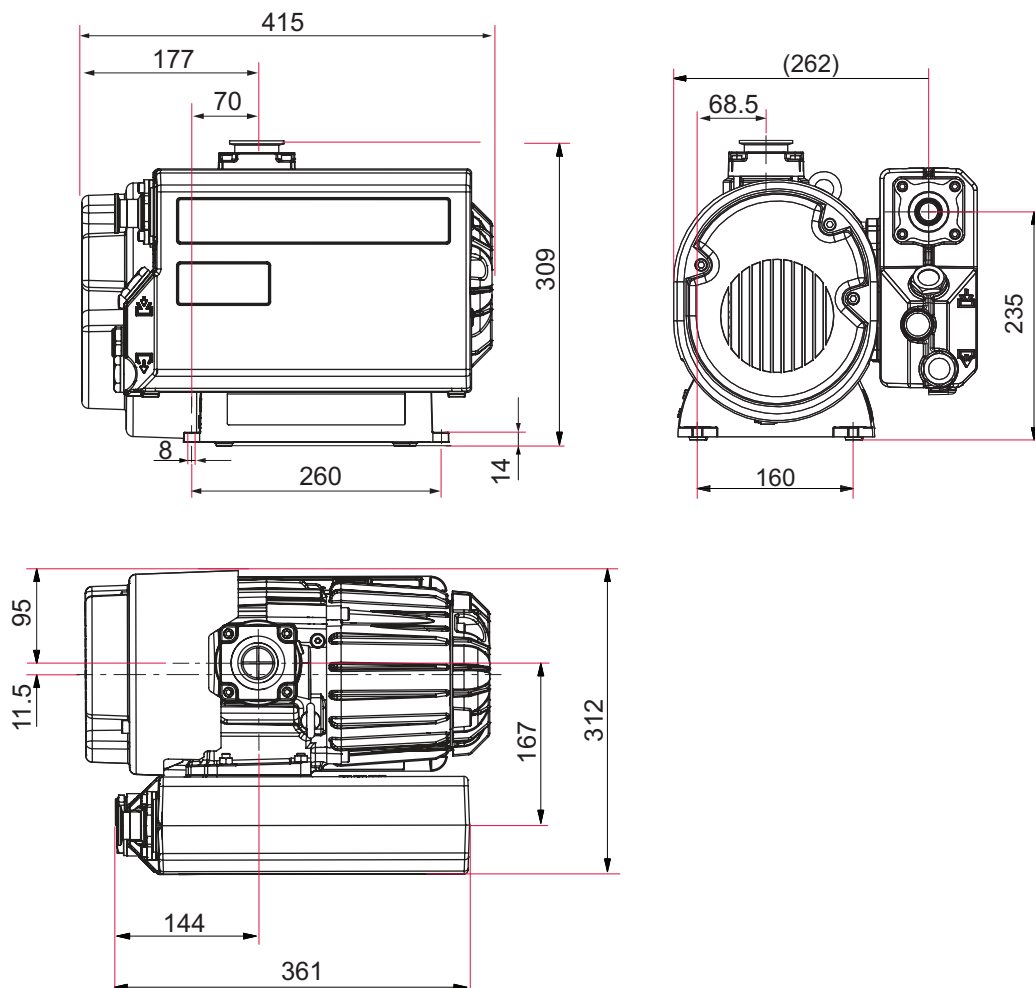
Fig. 17: Dimensions of SmartVane 55 with 1.75 l separator Dimensions in mm
