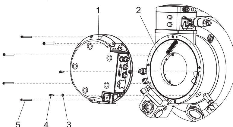
Fig. 28: Removing the electronic drive unit
