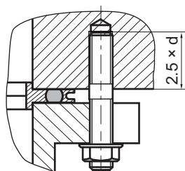
Fig. 16: Flange connection ISO-F, stud screw and tapped hole
