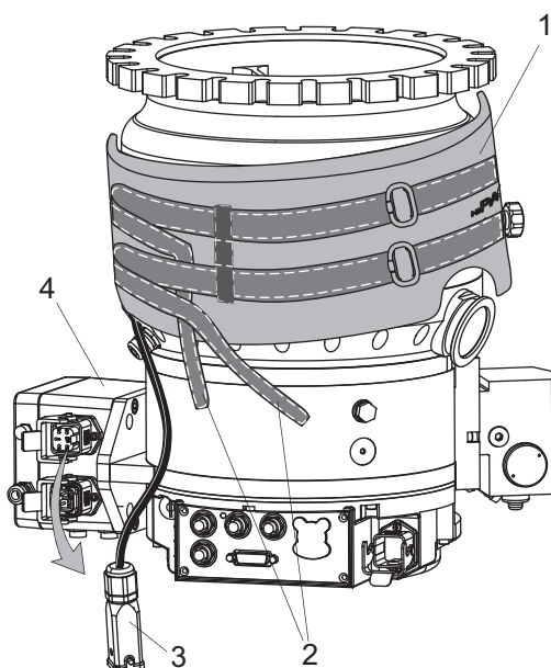
Fig. 30: Remove heating sleeve
