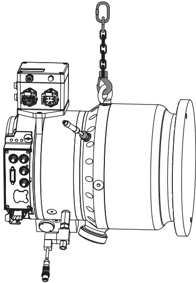
Fig. 5: Slings points for horizontal transport of the turbopump without packaging
