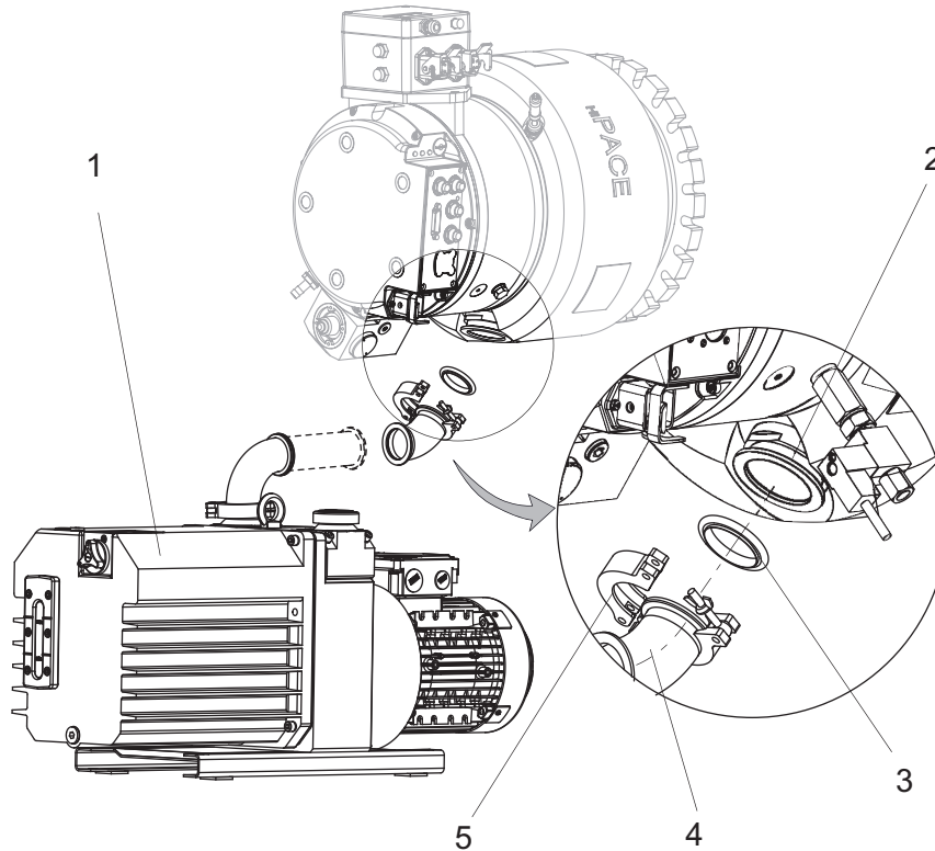
Fig. 20: Example of the fore-vacuum connection on the HiPace 1200 T
