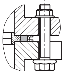
Fig. 15: Flange connection ISO-F, hexagon head screw and through hole
