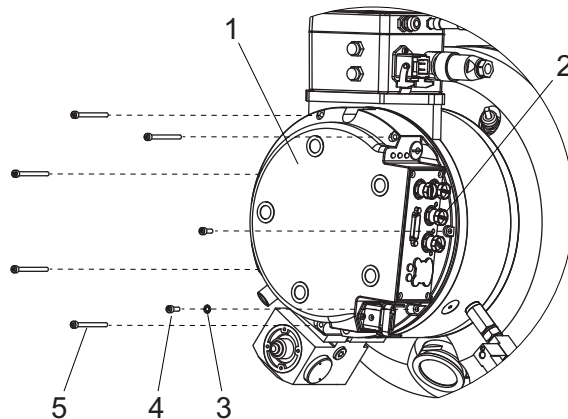
Fig. 29: Securing the electronic drive unit
