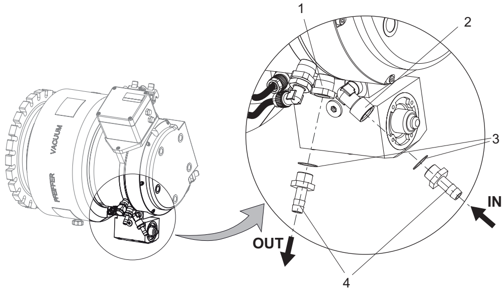
Fig. 21: Establishing a cooling water connection with hose nozzles
