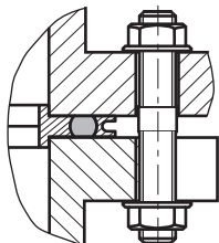
Fig. 17: Flange connection ISO-F, stud screw and through hole
