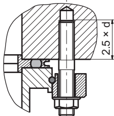
Fig. 12: Flange connection ISO-K to ISO-F, stud screw and tapped hole
