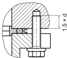
Fig. 14: Flange connection ISO-F, hexagon head screw and tapped hole
