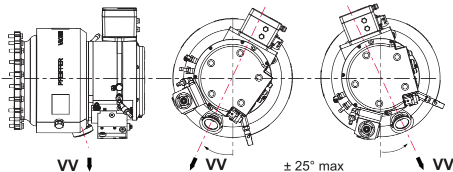
Fig. 9: Alignment of the fore-vacuum connection with horizontal mounting orientation
