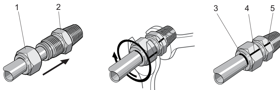
Fig. 33: Mounting the pipe fittings
