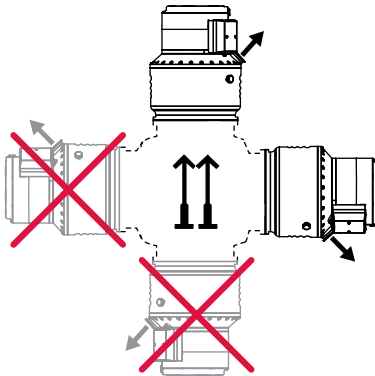
Fig. 8: HiPace 1200 | Mounting orientations of the U version, overhead
