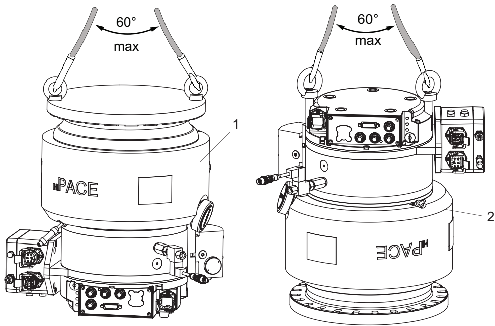
Fig. 4: Slings points for vertical transport of the turbopump without packaging
