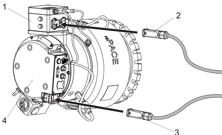
Fig. 24: Mains connection HiPace 1200 T
