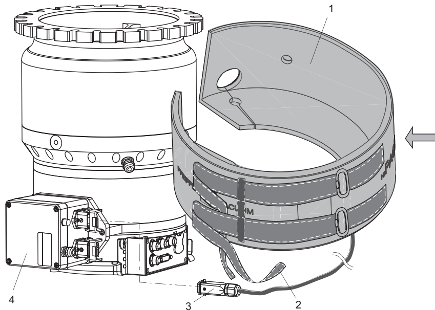
Fig. 31: Assemble heating sleeve
