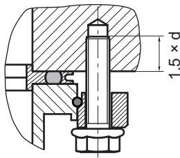
Fig. 11: Flange connection ISO-K to ISO-F, hexagon head screw and tapped hole
