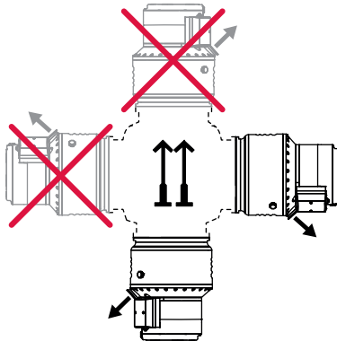
Fig. 7: HiPace 1200 | Mounting orientations of the standard version, upright
