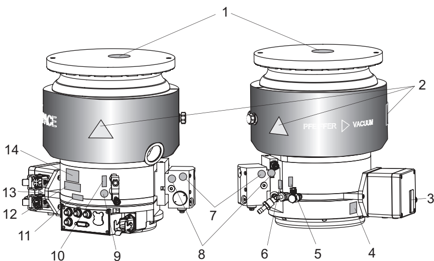
Fig. 1: Position of the stickers on the product
