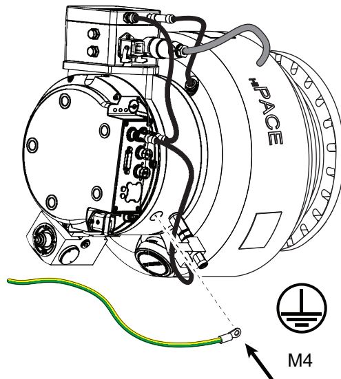
Fig. 23: Example: Connecting the grounding cable
