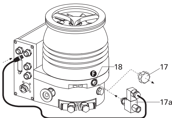
Fig. 7: Connecting the venting valve
