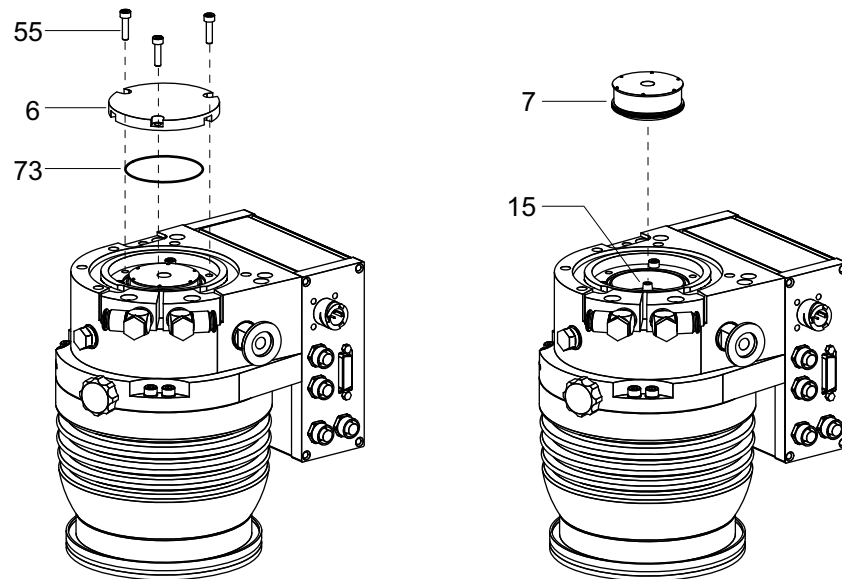
Fig. 12: Assembly / Disassembly of the operating fluid reservoir
