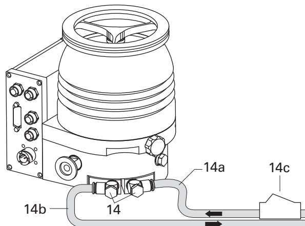
Fig. 10: Connecting the cooling water
