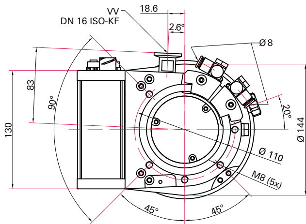
Fig. 15: HiPace 300 Plus, DN 100 CF-F
