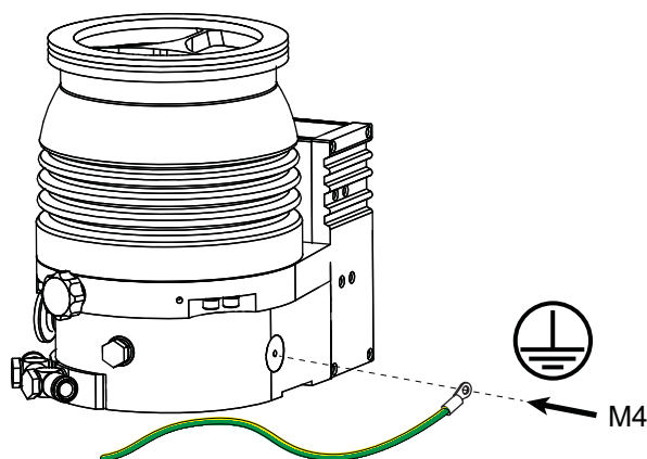
Fig. 5: Installing the earthing connection
