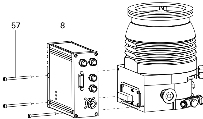
Fig. 13: Assembly / disassembly of the TC 400
