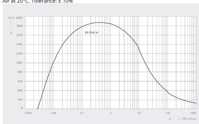
Pumping speed
